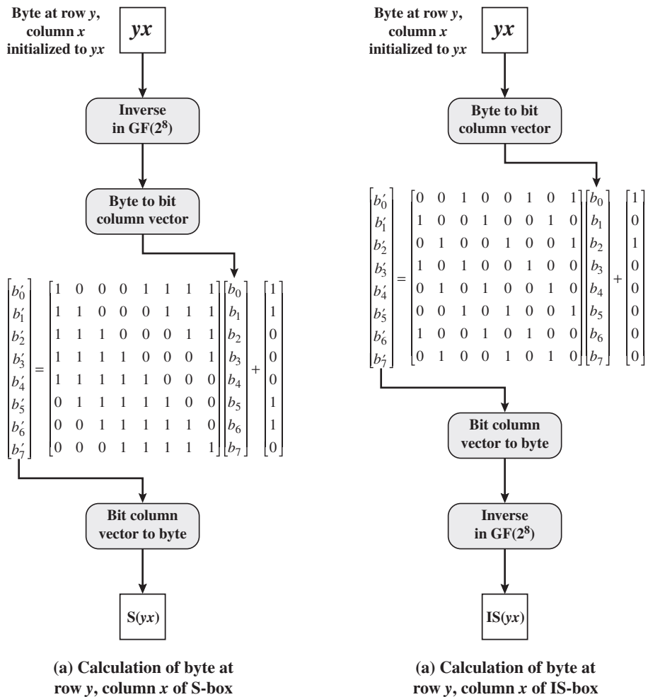
Figure 5.6 Constnction of S-Box and IS-Box
