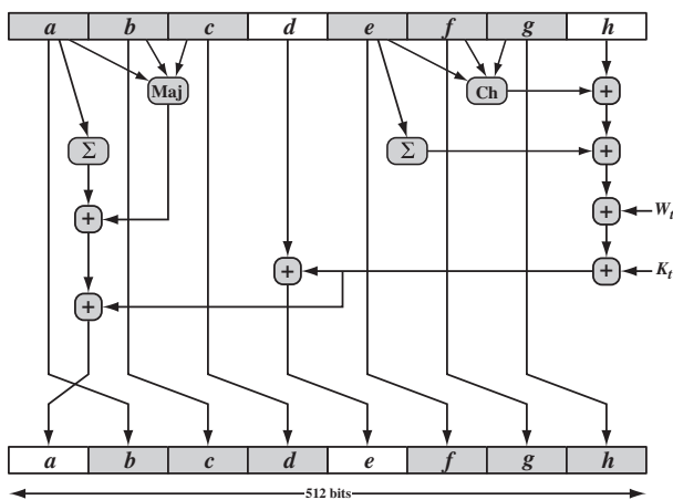
Figure 11.11 Elementary SHA-512 Operation (single round)
