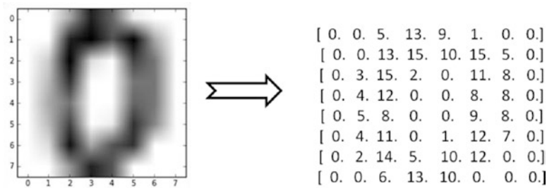
Figure 6-2. Handwritten digit(zero)image and corresponding array
