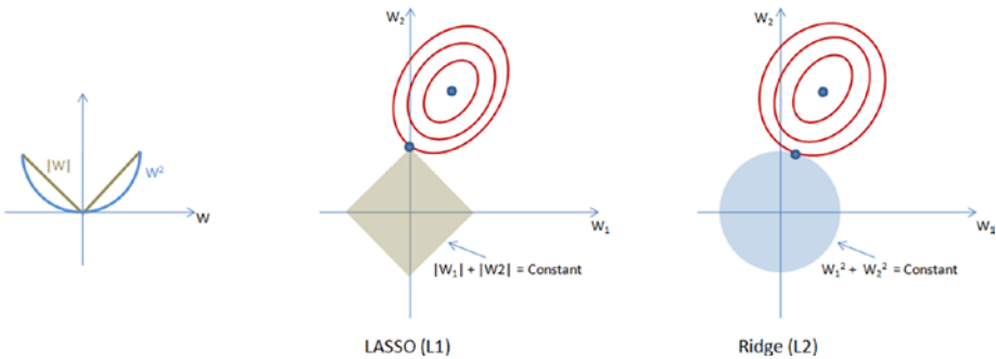
Figure 3-9. Regularizations
